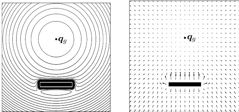
Fig. 12.14. The total potential in \mathcal{C} = \mathbb{R}^2 obtained by superposition of a hyperboloidic attractive potential and a repulsive potential for a rectangular \mathcal{C} -obstacle: left : the equipotential contours, right : the resulting force field
