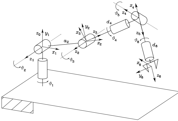
Fig. 2.26. Anthropomorphic arm with spherical wrist
