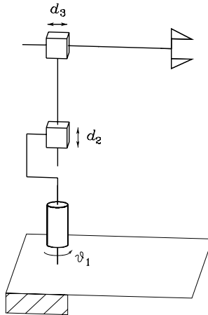
Fig. 2.35. Cylindrical arm
