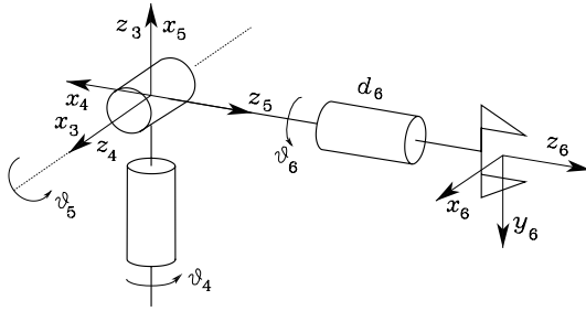
Fig. 2.24. Spherical wrist
