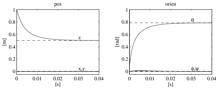
Fig. 10.9. Time history of camera pose estimate
