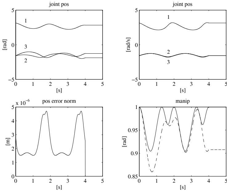
Fig. 3.19. Time history of the joint positions, the norm of end-effector position error, and the manipulability measure with the Jacobian pseudo-inverse algorithm and manipulability constraint; upper left : with the unconstrained solution, upper right : with the constrained solution
