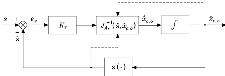
Fig. 10.7. Pose estimation algorithm based on the inverse of image Jacobian
