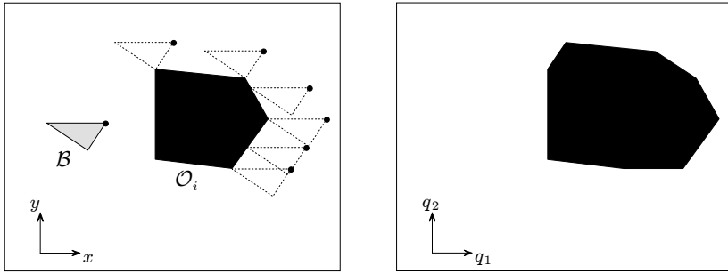
Fig. 12.3. \mathcal{C} -obstacles for a polygonal robot translating in \mathbb{R}^2 ; left : the robot \mathcal{B} , an obstacle \mathcal{O}_i and the growing procedure for building \mathcal{C} -obstacles, right : the configuration space \mathcal{C} and the \mathcal{C} -obstacle \mathcal{CO}_i
