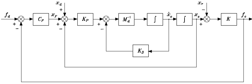
Fig. 9.8. Block scheme of parallel force/position control
