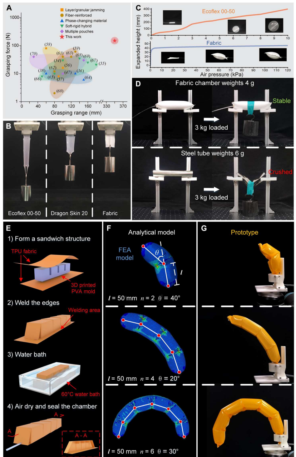
Fig. 1. Construction of the soft pneumatic actuators using soft, lightweight fabrics. (A) Comparison of the proposed fabric actuator-based gripper's grasping range and force with various previously developed soft grippers, including the ones with jamming parts (56–58), ones reinforced by fiber (59–63), ones integrated with phase-changing materials (36, 38, 64), ones with soft-rigid hybrid structures (54, 55, 65–68), and ones consisting of multiple pouches (47, 69, 70). (B) Responses of different soft pieces to the same tensile load. The passive stretching of the fabric piece is negligible compared with those of silicone rubber pieces. (C) Expanded height versus input pressure of a silicone-based airbag and a fabric-based one. As the pressure increases, the fabric-based airbag rapidly reaches its saturation point without future obvious height increase, while the silicone-based one continues to expand until the explosion. (D) Bending comparison between a fabric pneumatic cylinder and a steel tube with similar mass and identical size. The steel tube is readily crushed by a 3-kg weight, while the fabric chamber keeps stable upon the same payload under 45-kPa pressure. (E) Fabrication process of the fabric actuator. Step 1: Two pieces of thermoplastic polyurethane (TPU)-coated fabric are tightly attached to the 3D printed polyvinyl alcohol (PVA) mold. Step 2: Weld the overlapped fabric edges with an electric soldering iron. Step 3: Dissolve the internal PVA mold in 60°C water. Step 4: Air dry and seal the chamber together with a pneumatic pipe. The internal structure is shown in the bottom right corner. (F) Simulated deformation statuses of different actuators with various body lengths and rotation angles. These deformations can be predicted through both the finite element analysis (FEA) and a theoretical model based on robot kinematics. (G) Actual deformation statuses of three actuators with geometric parameters same as the simulated ones.
