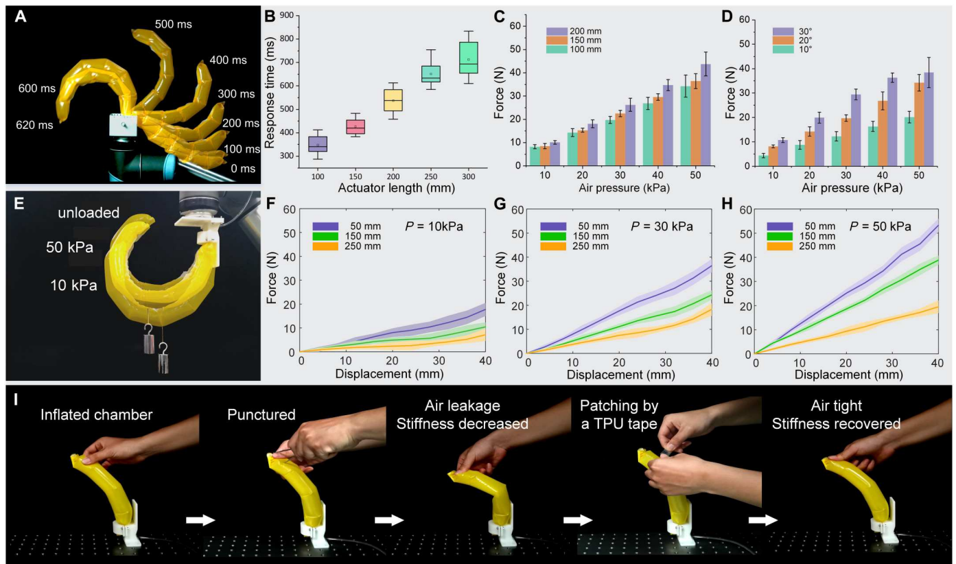
Fig. 2. Mechanical properties of the fabric actuator. (A) Response of a 250-mm-long actuator upon inflation. (B) Required times for reaching deformation limits. Five actuators with body lengths between 100 and 300 mm were tested. (C) Tip blocked force of three actuators in different body lengths at different pressure values. (D) Tip blocked force of three actuators with different rotation angles at different pressure values. (E) Comparison of an unloaded bending actuator and a 1-kg loaded actuator with input pressure of 10 and 50 kPa. (F to H) Stiffness curves of actuators in different body lengths at different pressures. Actuator stiffness showed positive correlation with pressure and negative correlation with body length. (I) Simple, quick repair process of a leaked/damaged actuator. The patched actuator can almost restore to its original performance.
